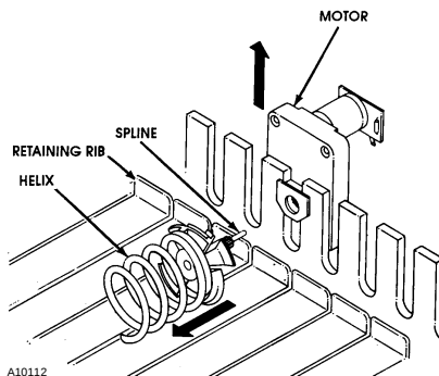
Figure 12. Auger Motor assembly
