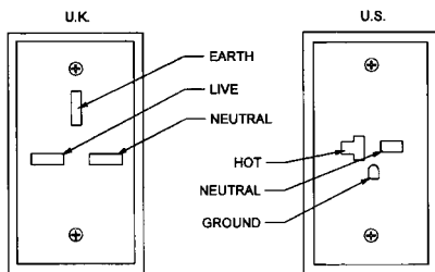
Figure 5. 230-Volt Outlets
