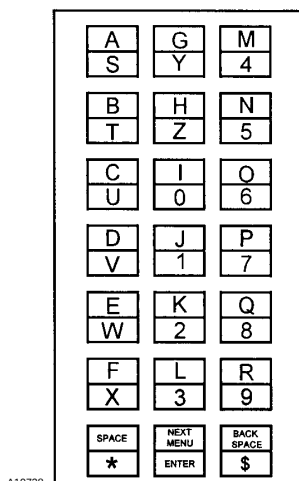
Figure 13 Keypad Overlay
