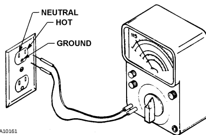
Figure 7. Electrical Check with Voltmeter
