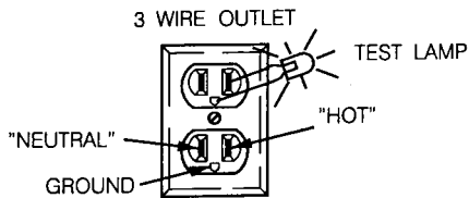
Figure 6. 115-Volt Outlet
