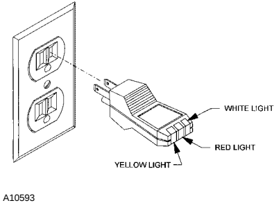
Figure 8. 3-Prong Outlet Tester
